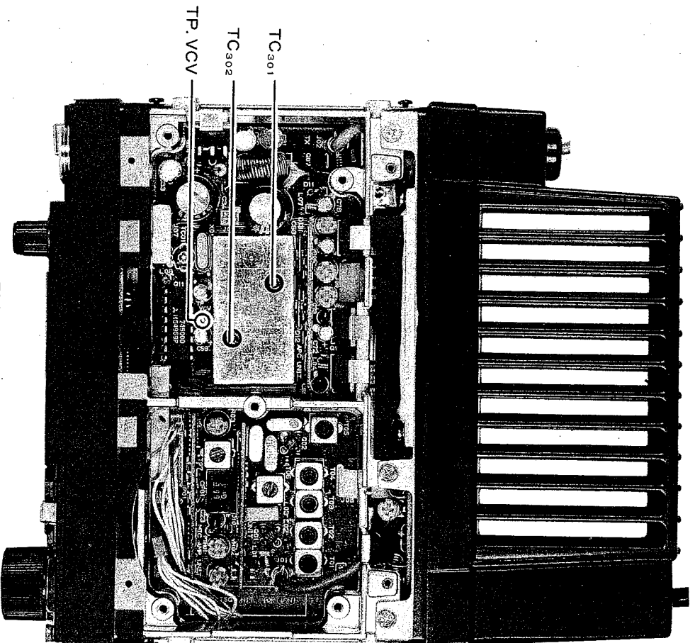
PLL ALIGNMENT POINTS
